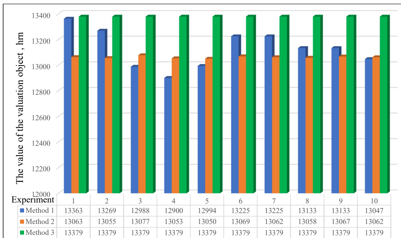
Figure 1 – The results of a computational experiment on the sensitivity of mathematical methods for the implementation of a comparative approach in real estate valuation in relation to the procedure for digitizing the initial data
