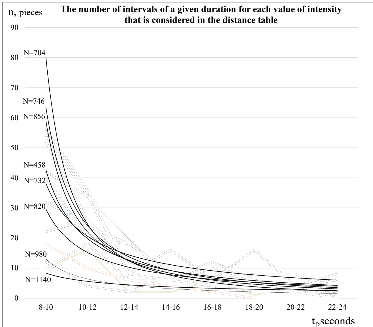
Figure 2 – Graph of the number of intervals of the given duration for each intensity value, which was considered in the study. Where t_f is the duration of the free interval, seconds; n - the number of free intervals of a given length, pieces; N - traffic intensity, cars / hour.
