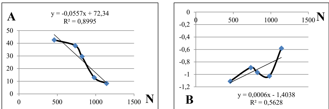
Figure 3 – The graph of the coefficient A and coefficient B dependence on the traffic intensity N.
