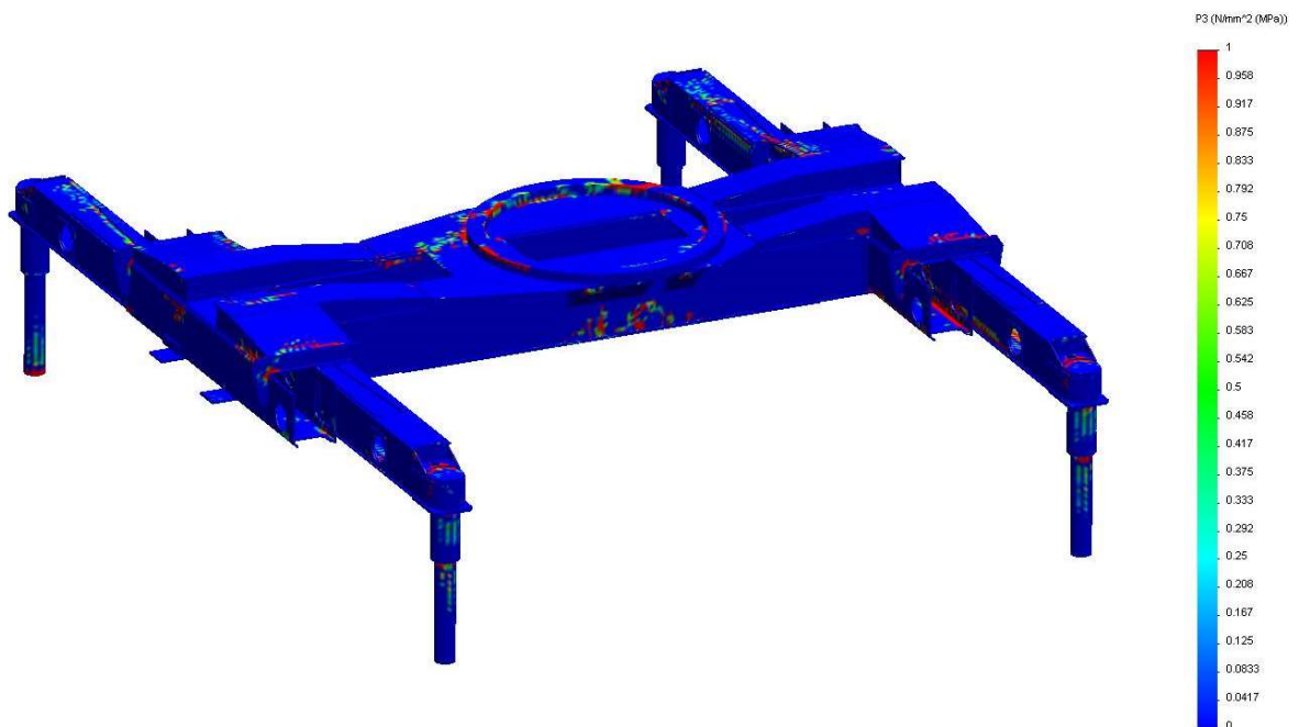
Figure 4 – The result of the calculation of the crane frame
